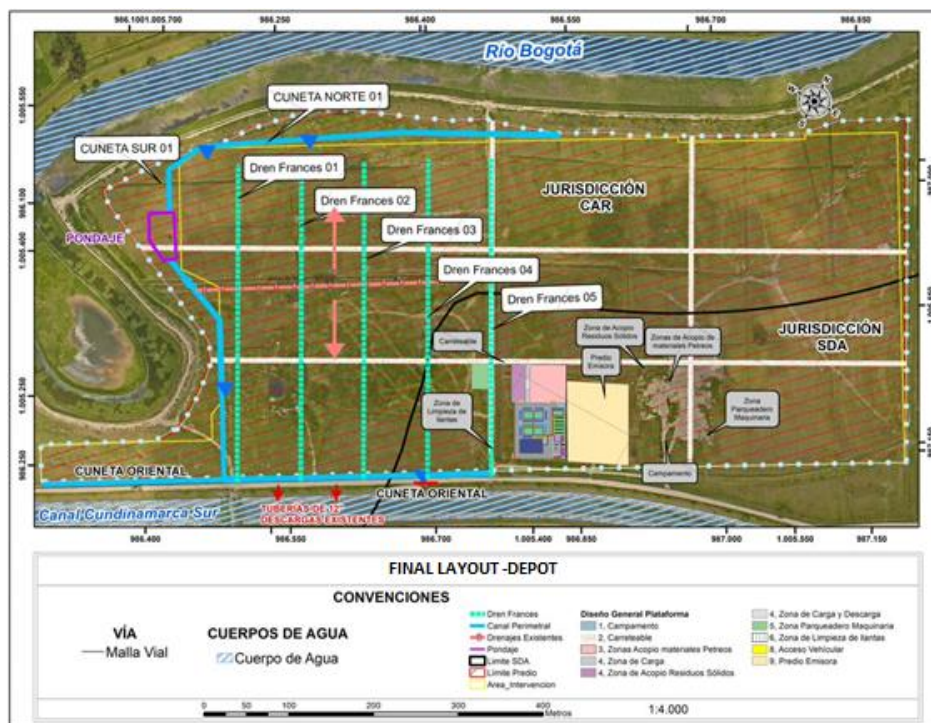
Figure 7 Final Depot Layout
